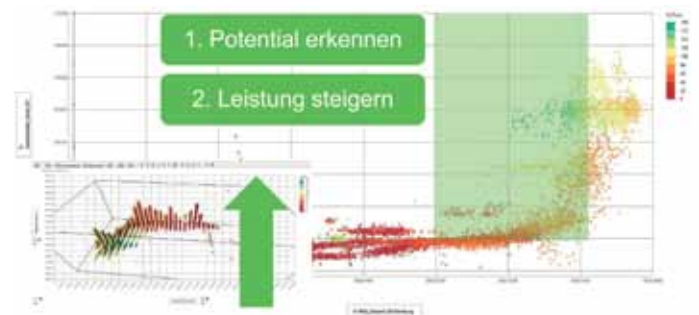
RevoOptimizer Analyse
