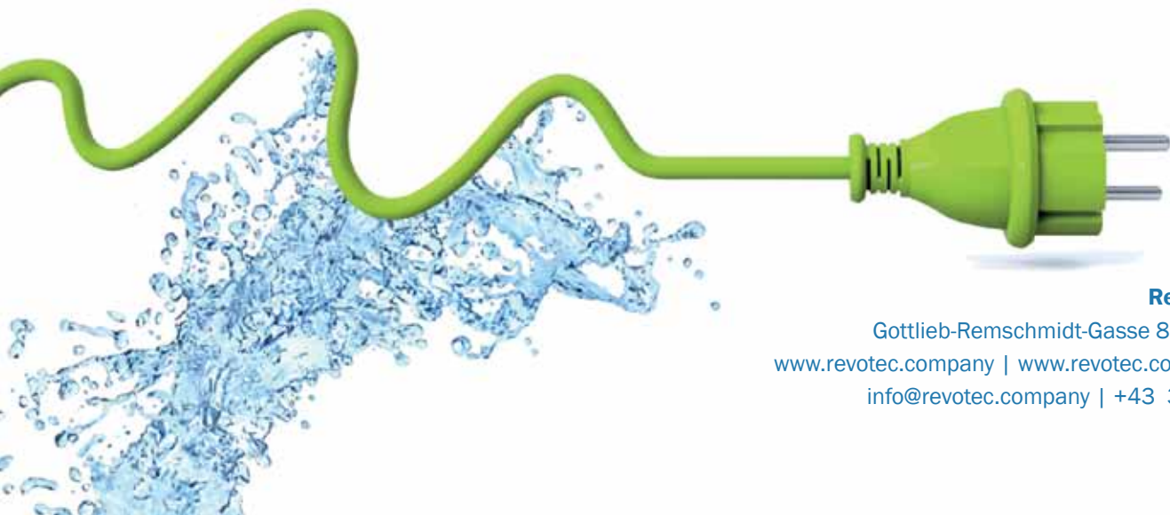
RevoOptimizer Analyse
